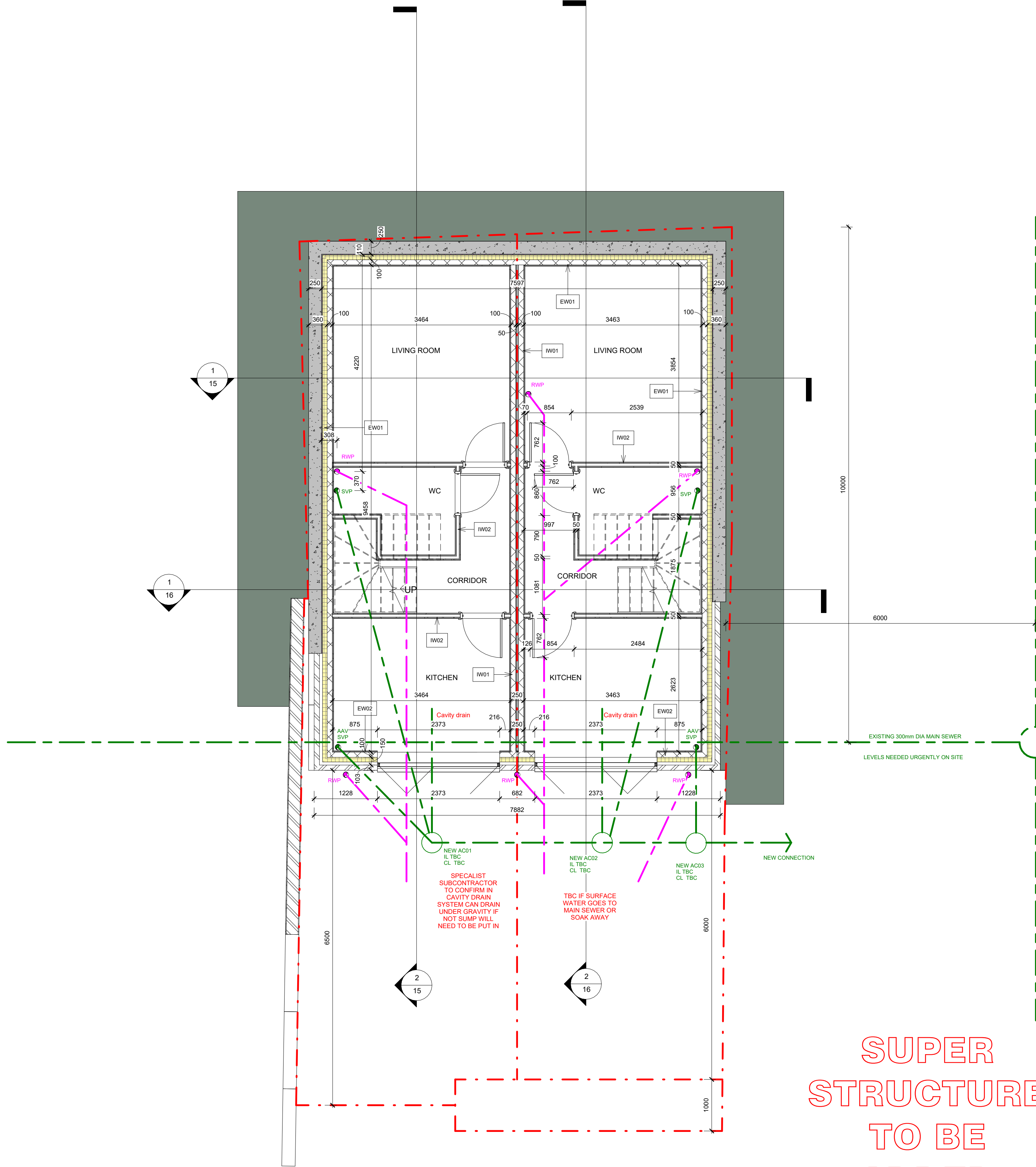
2 Lower Ground Floor 1 : 50
