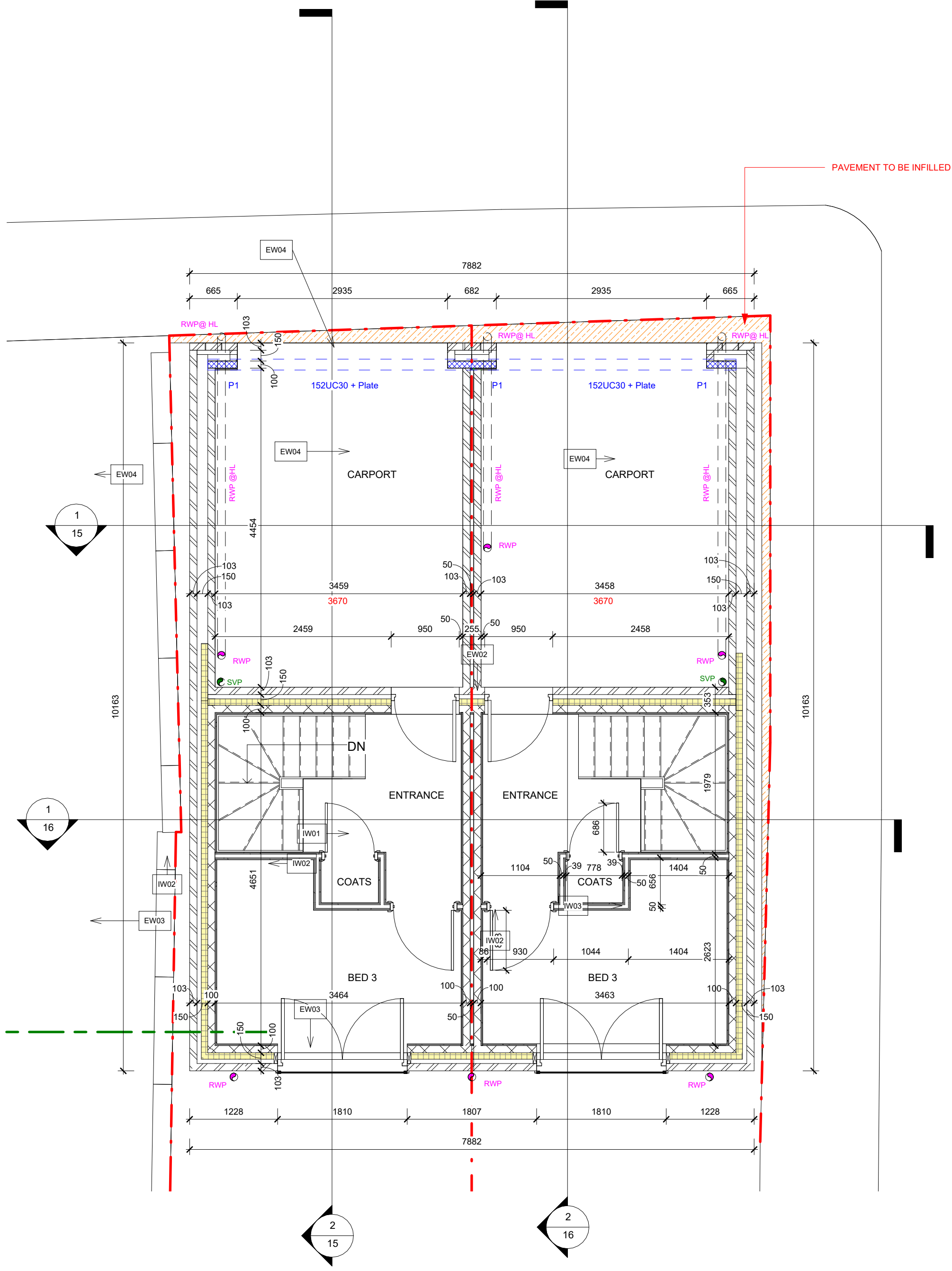
1 Ground Floor 1 : 50
